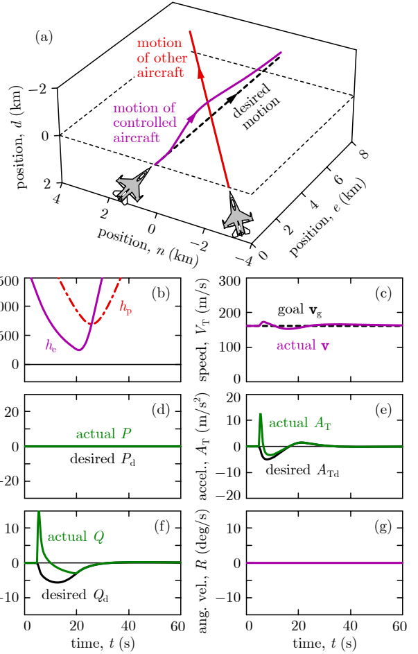
Fig. 3. Simulation of RTA in collision avoidance using extended CBF. The aircraft successfully maintains safety.
